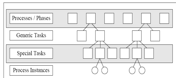
Figure 1: Four Level Breakdown of Data Mining
