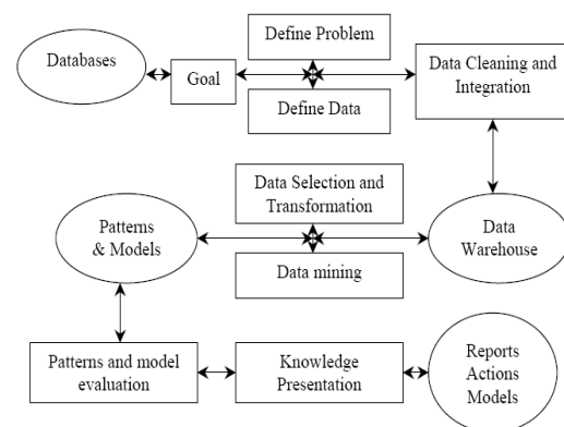
Figure 2: Complete KDD Process
