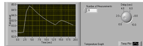
Figure 3: An example virtual instrument graphical user interface.
