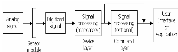
Figure 4: Sensory model.
