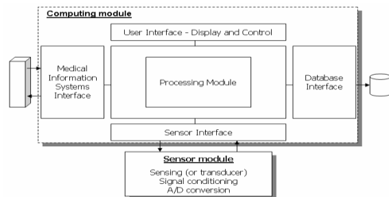
Figure 1: Architecture of a virtual instrument
