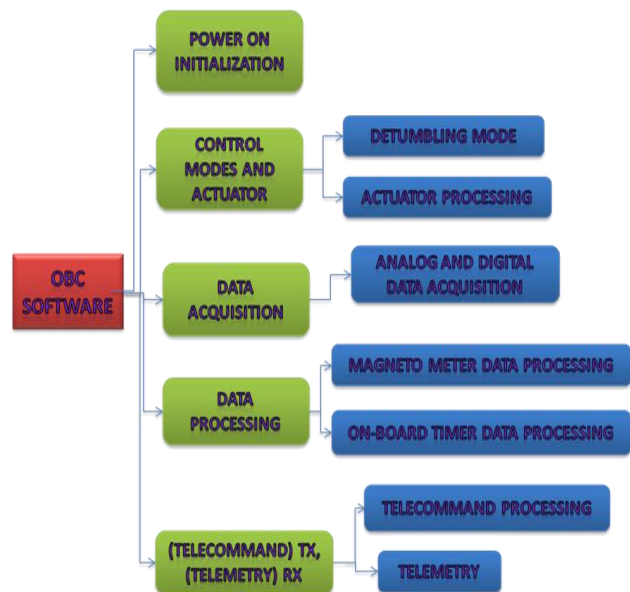
Figure 3: OBC Software Components
