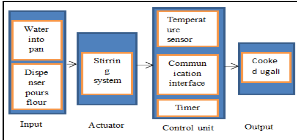
Figure 1 Block diagram of smart ugali cooker
