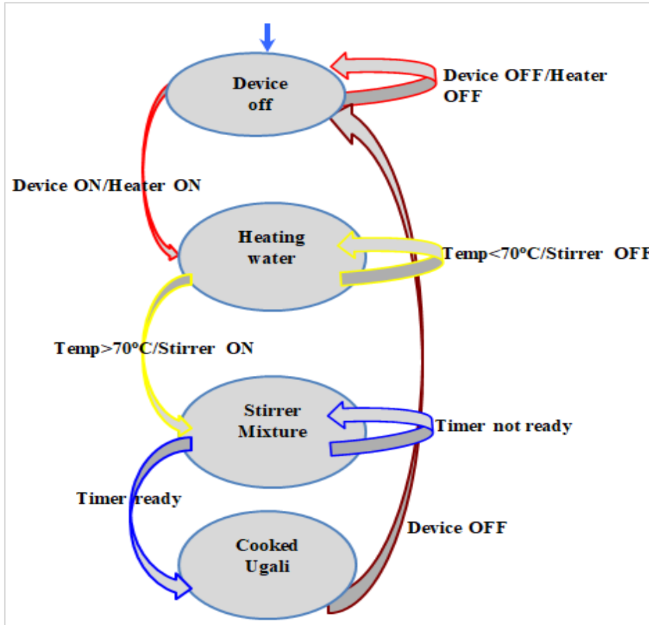
Figure 3 Finite state machine for ugali cooker
