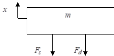
Figure 3 Damper and spring forces in car model
