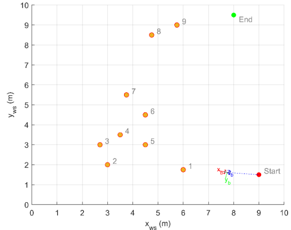
Figure 2 Navigation problem
